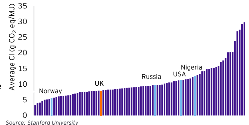
Estimated global upstream crude oil carbon intensity (2015)
