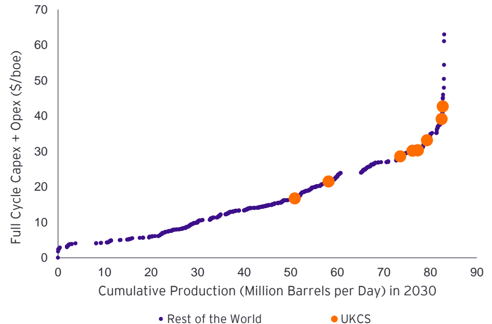
UKCS vs. Rest of the World cost curve - individual fields
